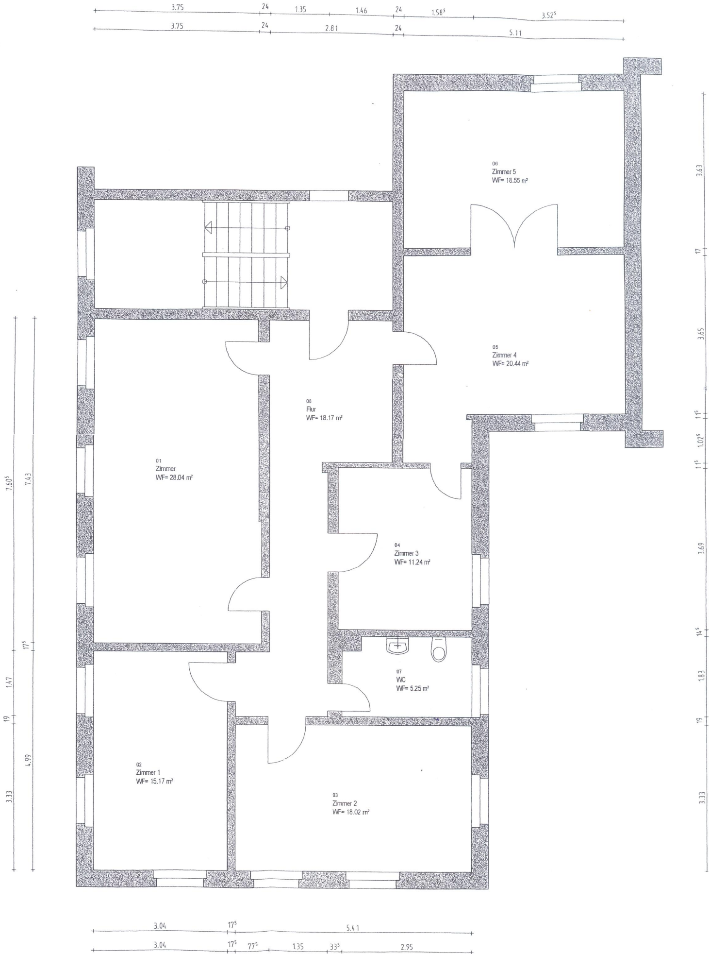
Goethestrasse 51, 1.Obergeschoss links = 134.88 m 2
